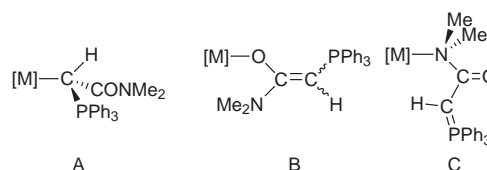
Scheme 2 Expected co-ordination modes for the ylide \text{Ph}_3\text{P}=\text{C}(\text{H})\text{CONMe}_2
